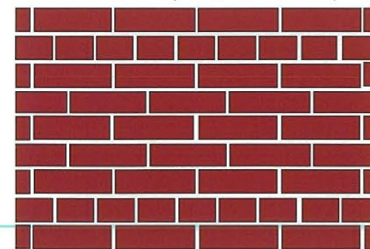
Common Bond (6th course headers)
