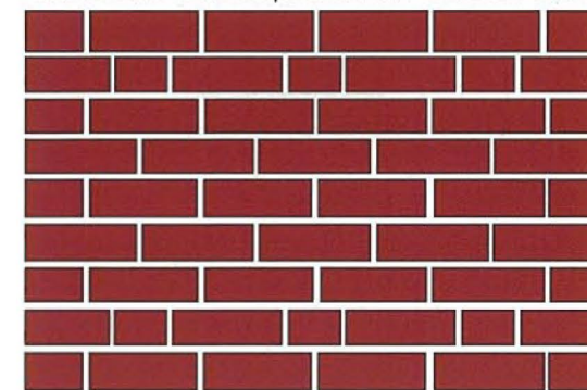
Common Bond (6th course Flemish headers)
